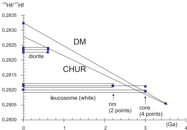
Figure 7. Hf isotopic evolution diagram. Figure show CHUR, DM (Vervoort and Blichert-Toft, 1999) and zircon sample evolutions curves. The archaic zircon cores have positive \epsilon_{\text{Hf}} suggesting a mantle source, but in the paleoproterozoic zircon rims the \epsilon_{\text{Hf}} are negative, therefore suggesting a crustal source (Table 3). The neoproterozoic zircon grains from the diorite present \epsilon_{\text{Hf}} very close to zero suggesting mantle source mixed with small crustal material contribution (Table 4). Hf isotopic data were obtained by LA-ICP-MS from TITech, Tokyo, Japan.
