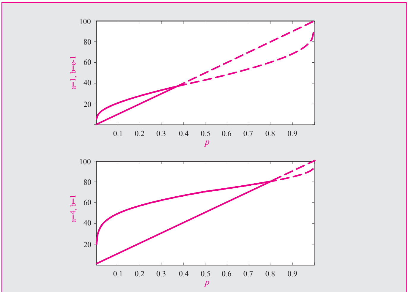
Figure 2: The Difference Between Expected Values of an Investment when Comparing the Adaptive Probability Theory Model with Expected Utility – Wrong Decision Regions
